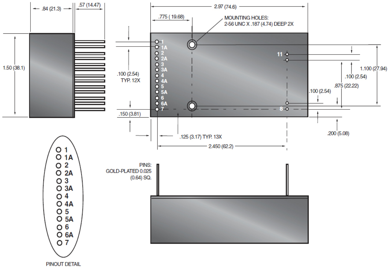
Figure 1 Outline Dimensions
