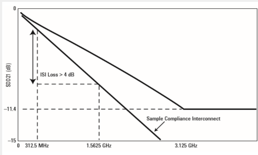
Figure 2. Today's digital standards are now using frequency domain measurements for compliance testing, such as this input differential insertion loss (SDD21) mask for XAU1
