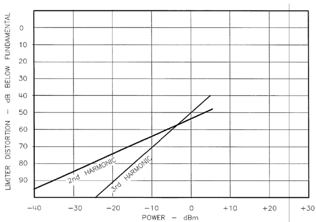
Figure 4 Typical harmonic distortion versus input power
