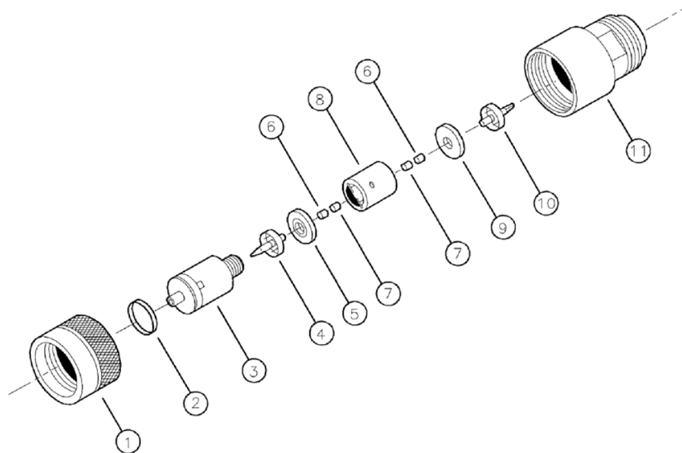
Figure 5 11867A illustrated parts breakdown
