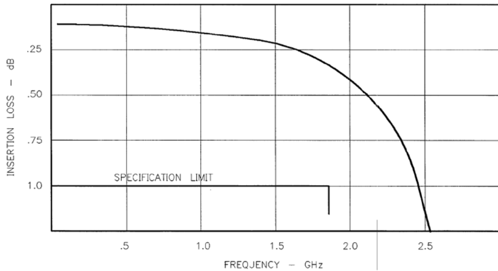
Figure 1 Typical insertion loss versus frequency
