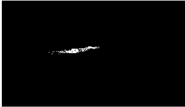
Fig. 6: Track generated by an \alpha -particle.
