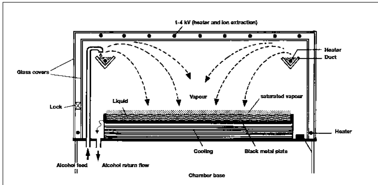
Fig. 2: Section through diffusion cloud chamber.
