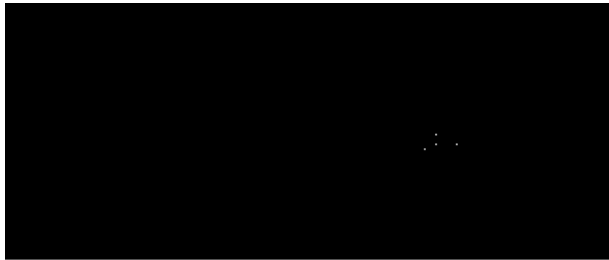
Fig. 13: Track of dissociation of a \mu -meson into an electron and two neutrinos.
