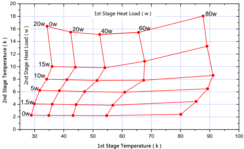
KDE415 Typical Load Map ( 50Hz )
