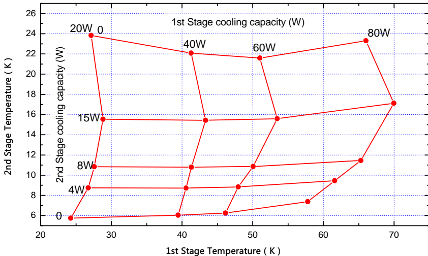
KDE210 Typical Load Map ( 50Hz )
