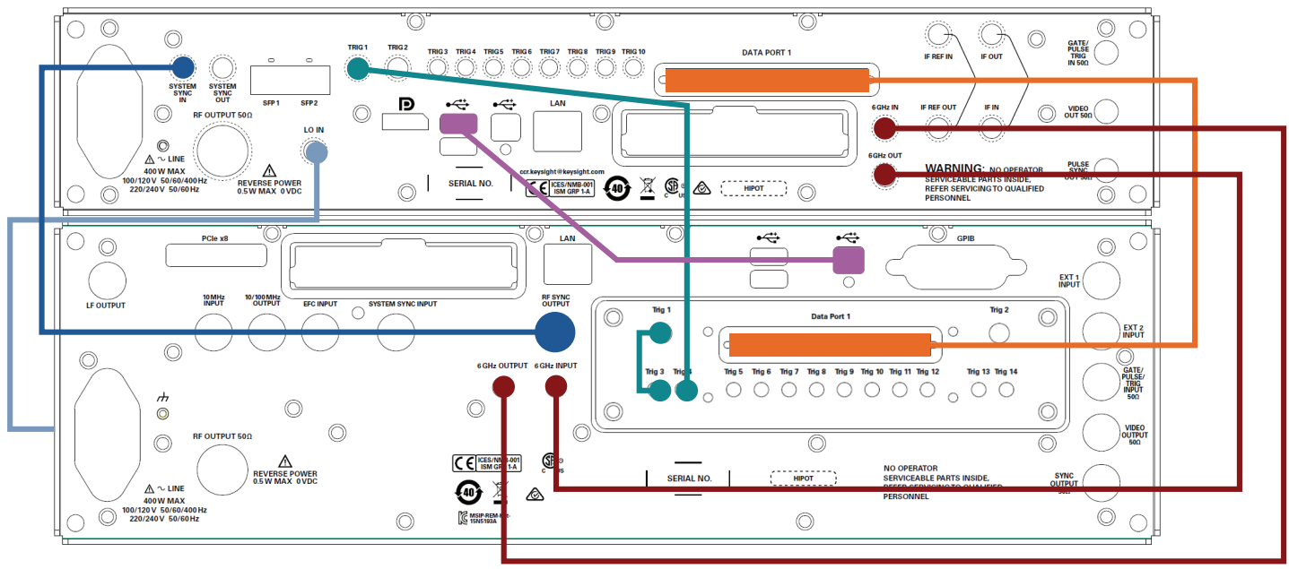
Figure 14. Connections between the XUG agile vector adapter and the XUG agile signal generator 1, 2 .
