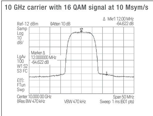
Spectral re-growth (measured)
