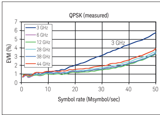
EVM (measured)
