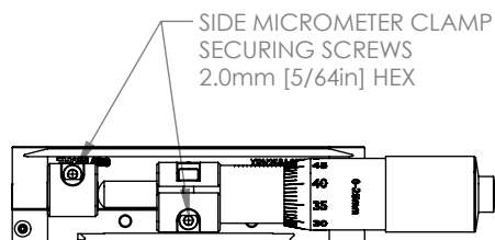
AUXILIARY SIDE VIEW
