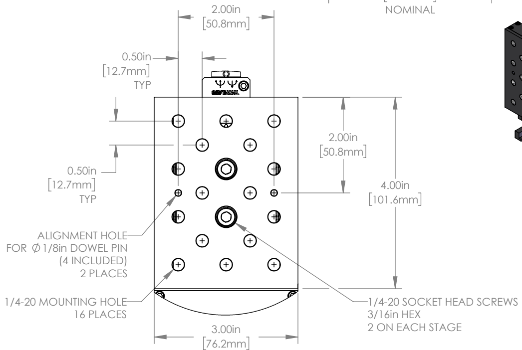
DETAIL A
