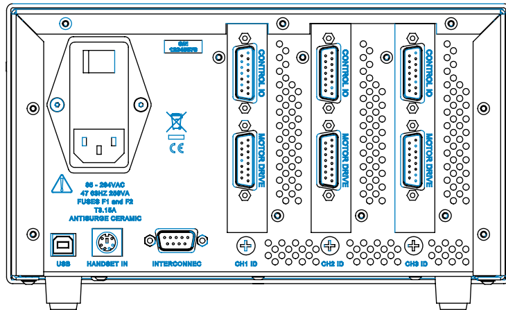
REAR PANEL VIEW
