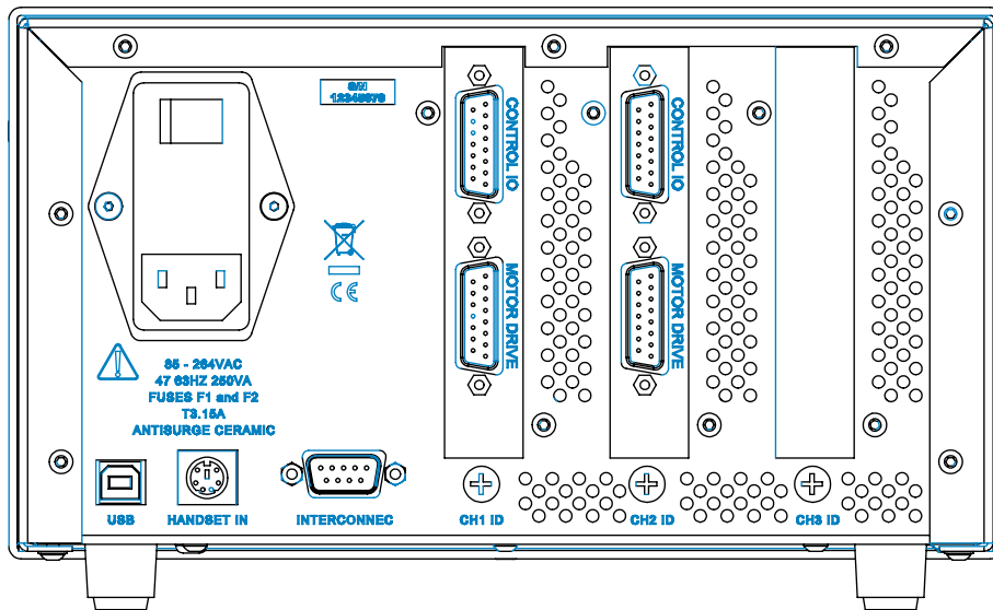
REAR PANEL VIEW
