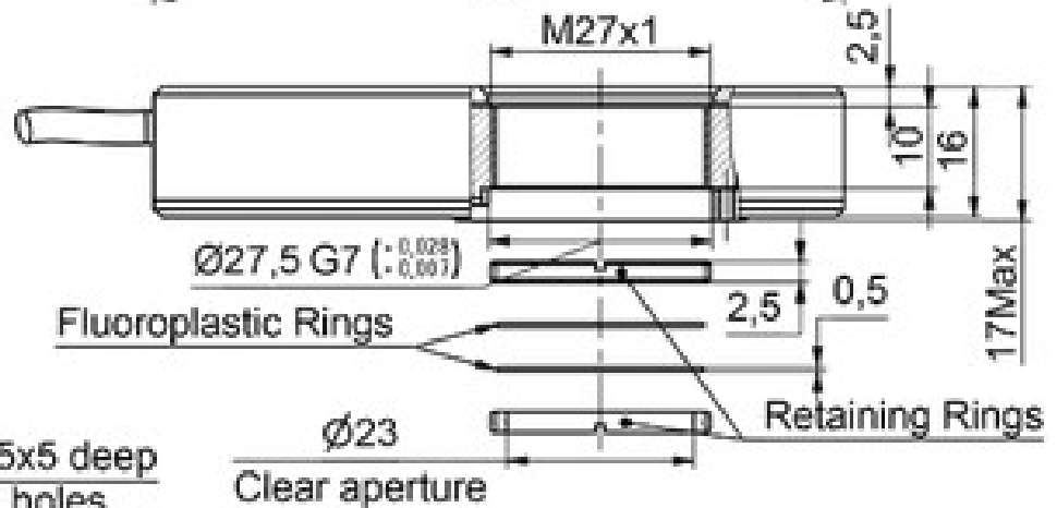
View A ( 1 : 2 )
