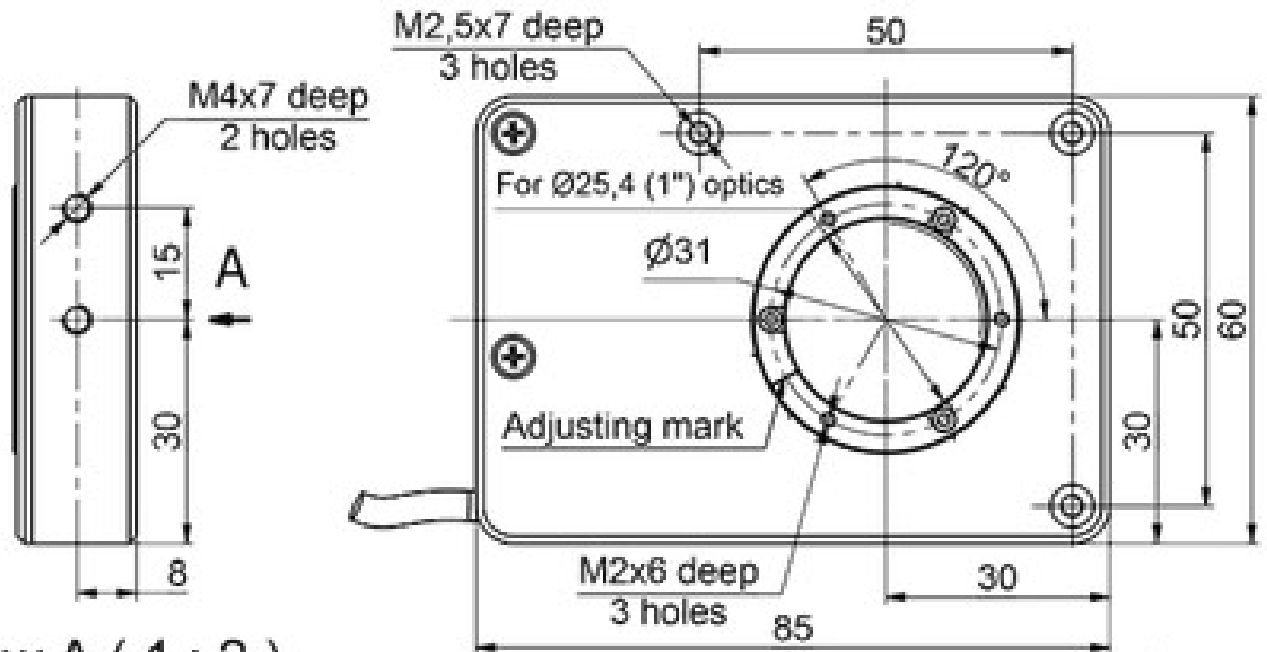
View A ( 1 : 2 )
