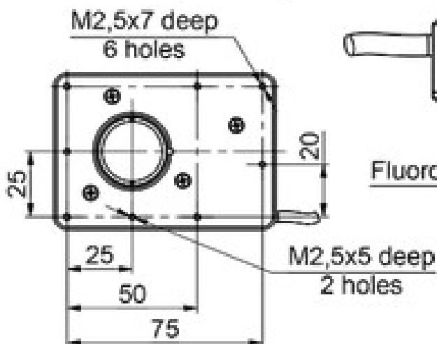
View A ( 1 : 2 )
