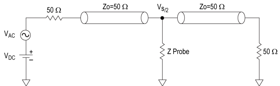
Figure 11: P76TA adapter simplified schematic
