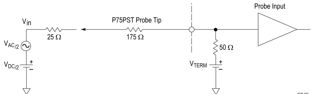
Figure 12: P76TA adapter and P75PST tip equivalent schematic
