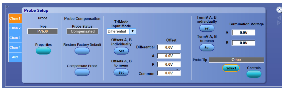
Figure 4: Typical TriMode Probe Setup screen
