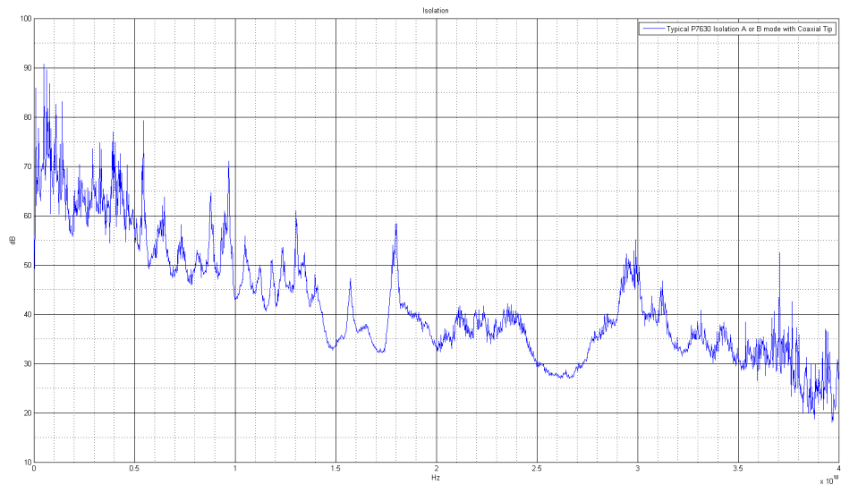
Figure 23: Typical channel isolation
