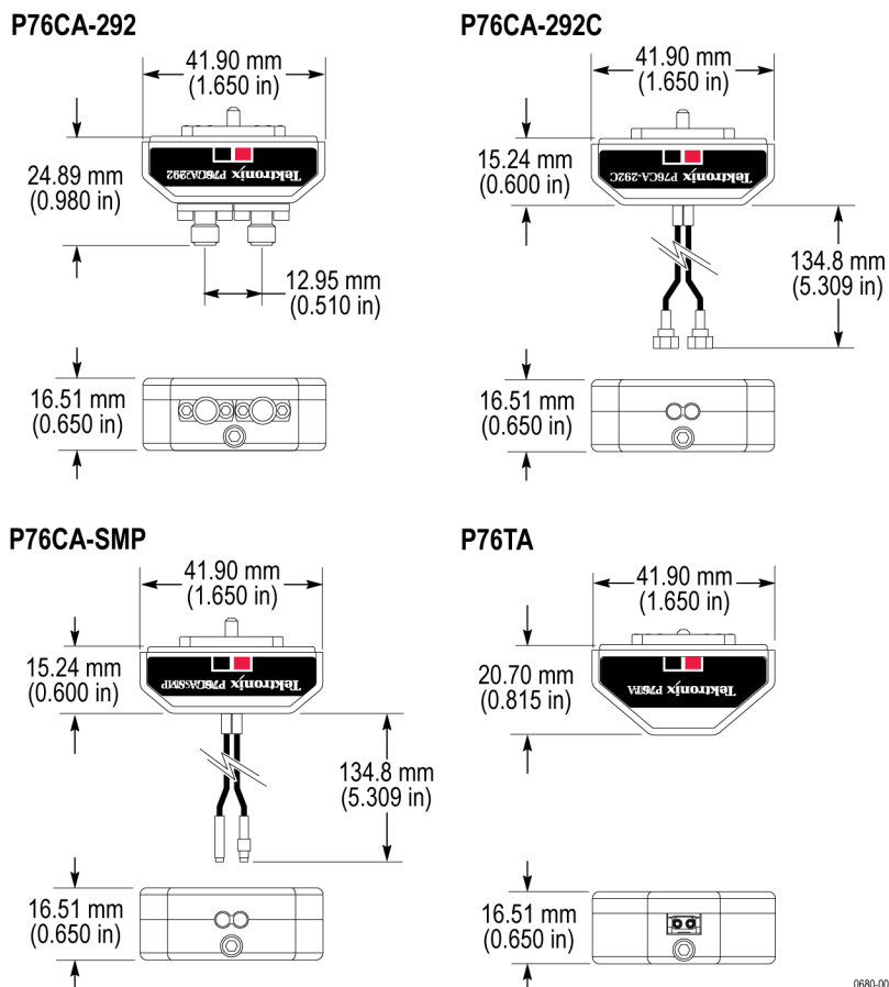
Figure 27: P7600 Series Probe adapter dimensions
