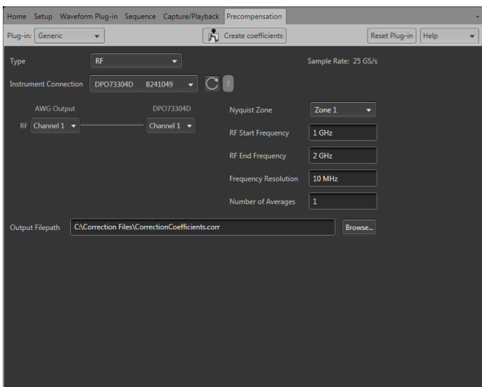
The AWG70000B with the Generic Precompensation plug-in
