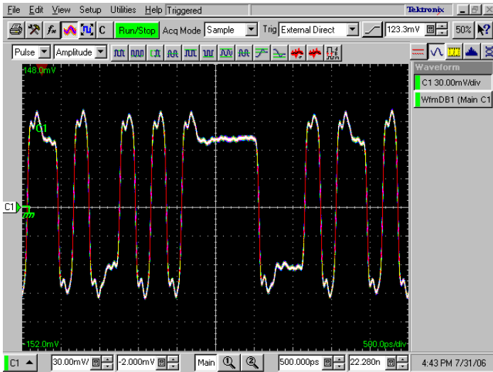
Digital data with de-emphasis added using the AWG70000B and the HSS plug-in
