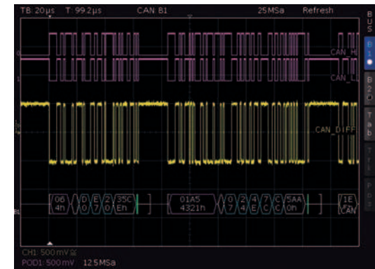
HEX decoded CAN bus signal
