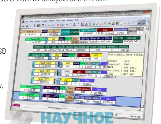
The CATC Trace display uses collapsible headers to group all packets that are part of a single transfer
