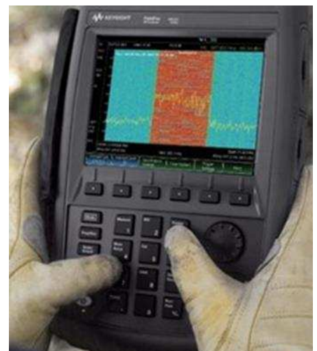
Easily operate FieldFox, even when wearing gloves, through the large front panel keys
