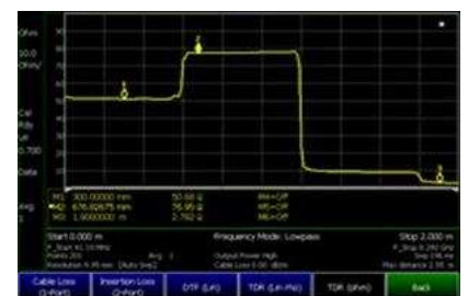
Gain insight into faults with TDR measurements
