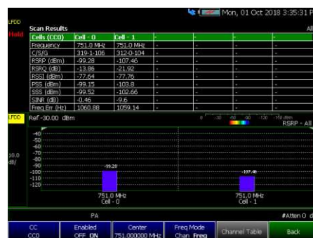
Multicell measurement with cell ID on single carrier frequency
