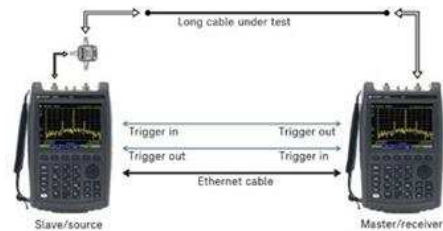
Measure long, lossy cables using ERTA
