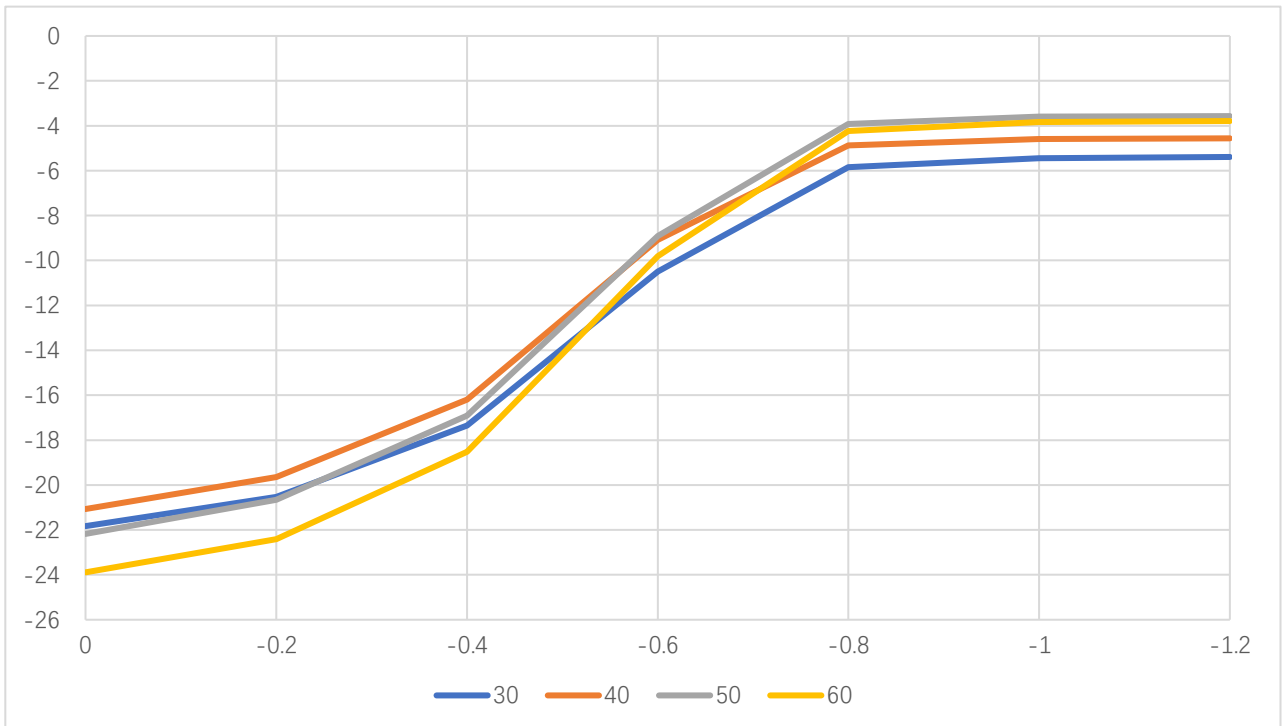
Attenuation vs Voltage at 30/40/50/60GHz
