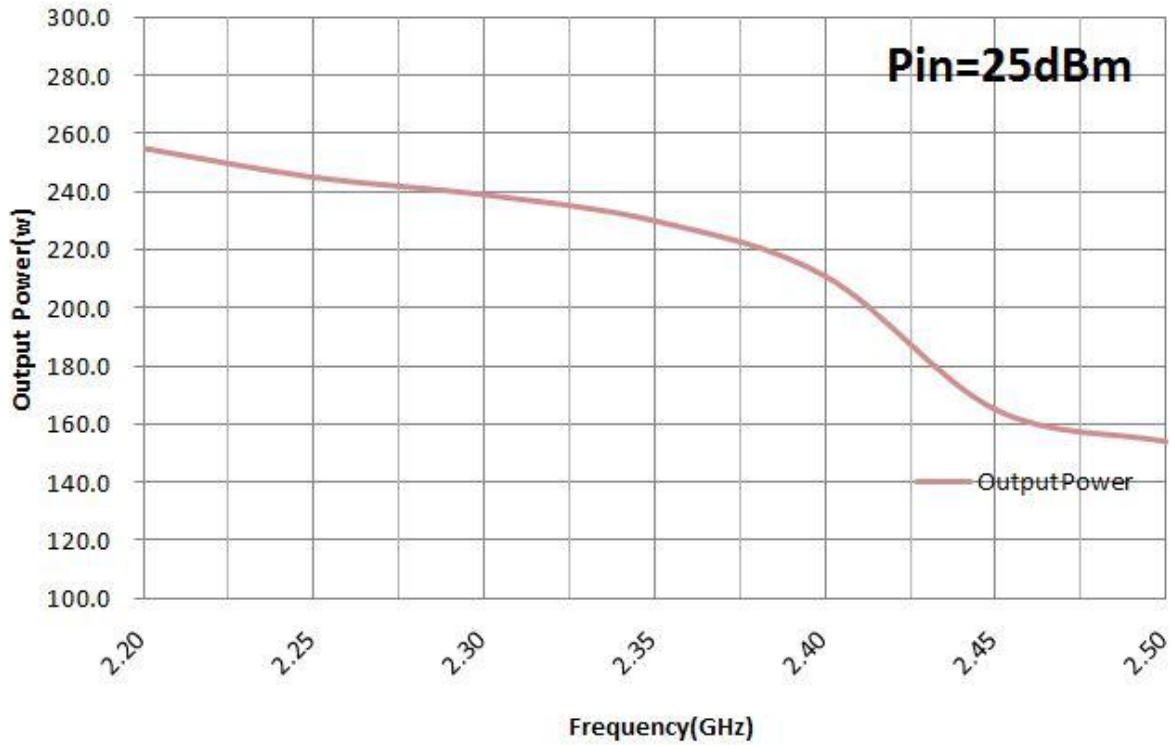
Graph1: Output Power(Normal temp.+25±3℃)
