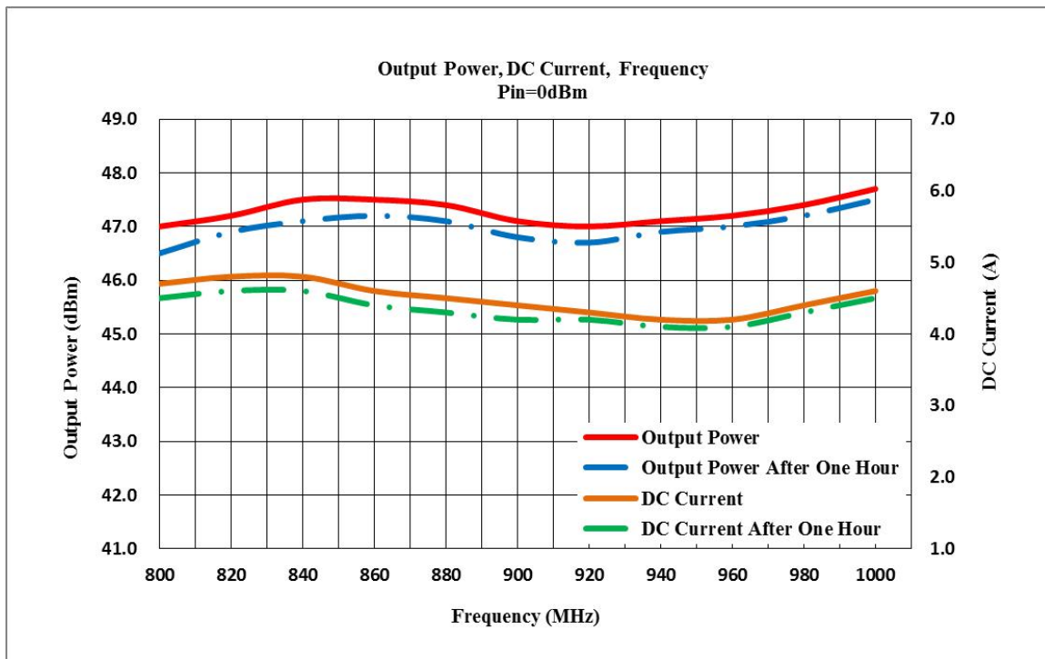
Graph2: Output Power(High temp.+60±3℃)
