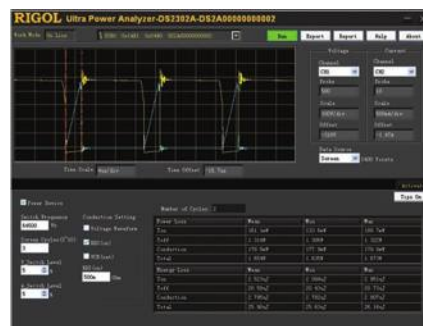
Power device switching loss analysis
