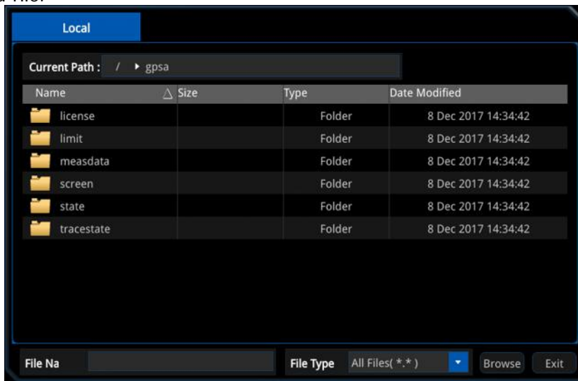
Figure 6-2 File Manager
