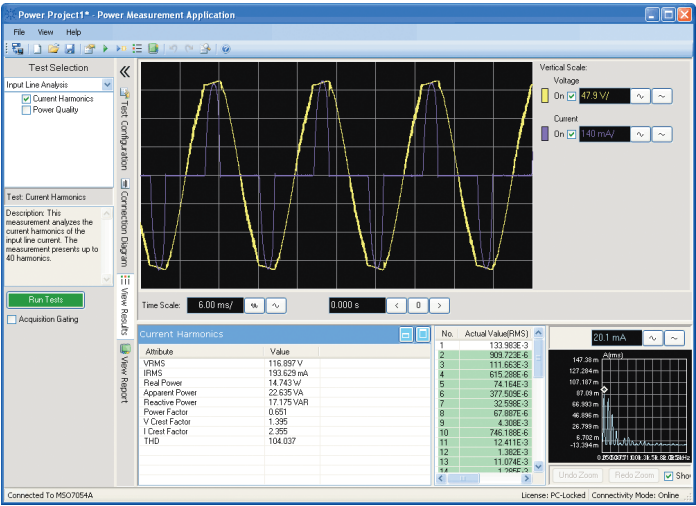
Figure 5. Input line analysis results.
