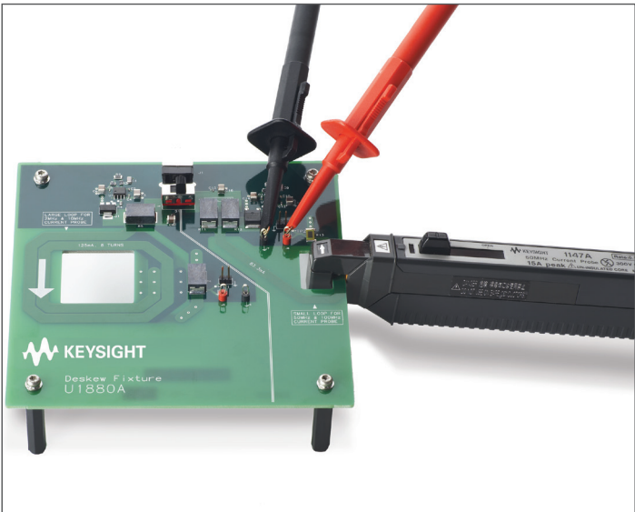
Figure 3. Deskew fixture.
