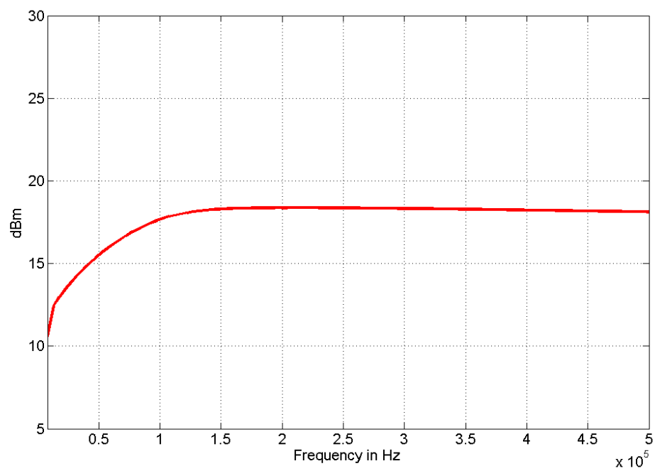
Figure 7. Maximum output power 8 kHz to 500 kHz (Option MFE)
