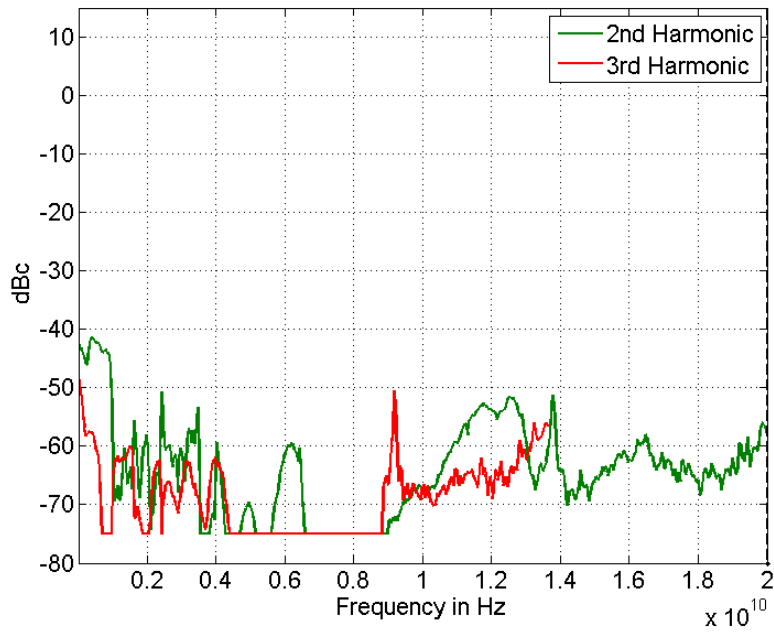
Figure 2. Harmonics (at 10 dBm output power)
