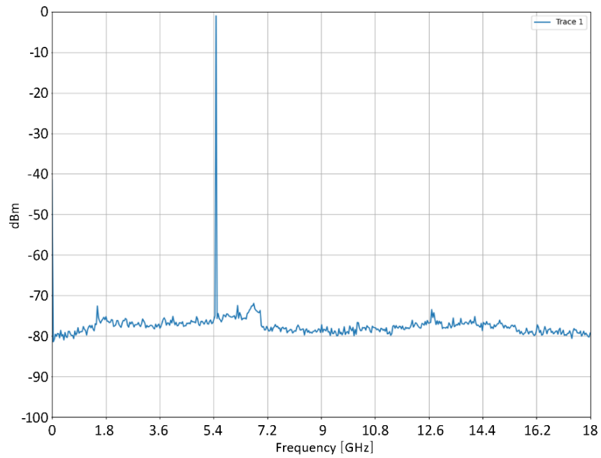
Figure 4. Wideband spectrum for 5 GHz
