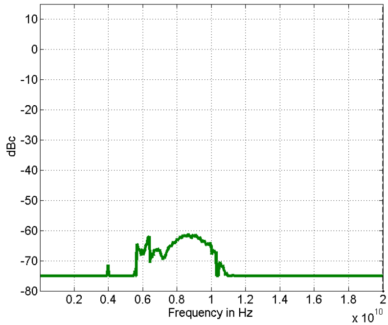
Figure 3. Subharmonics (at 10 dBm output power)
