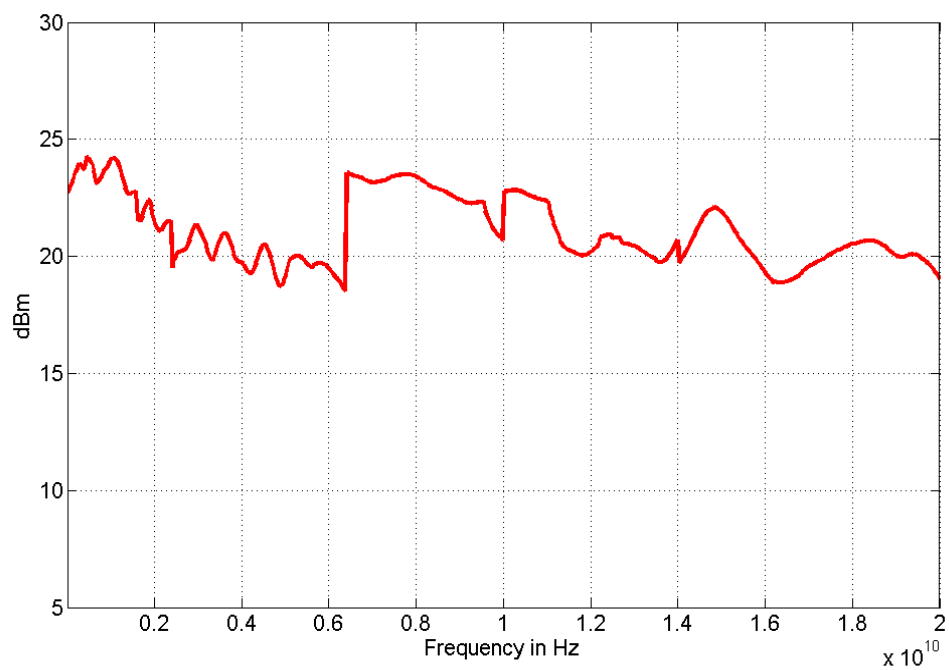
Figure 6. Maximum output power
