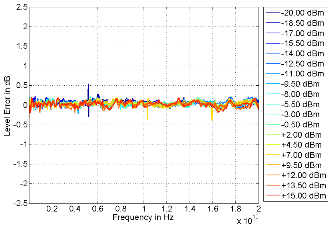
Figure 9. Frequency response
