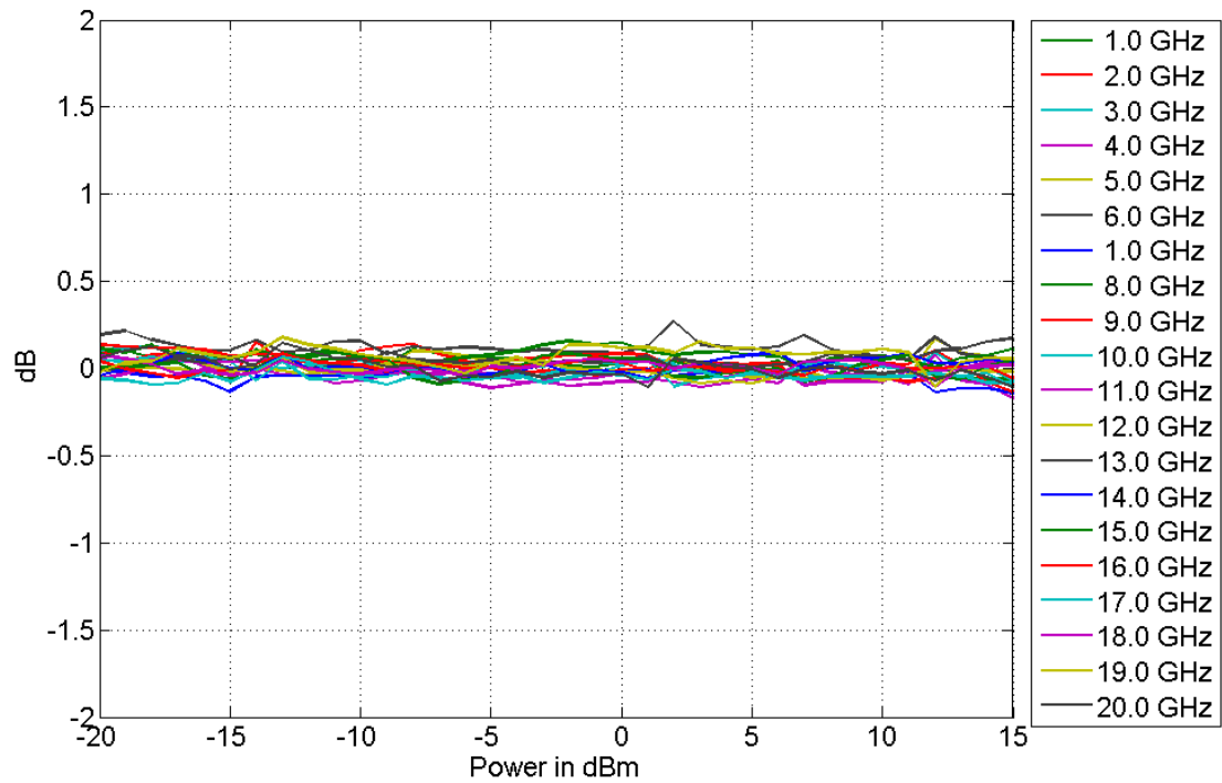
Figure 8. Power level linearity
