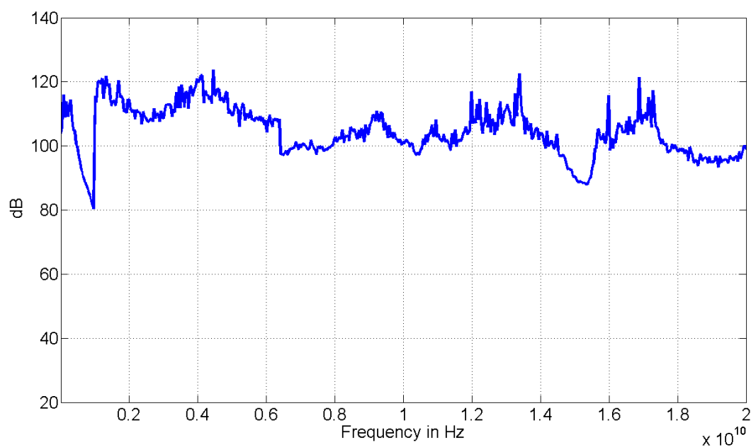
Figure 10. On / off ratio — pulse modulation (at 10 dBm output power)
