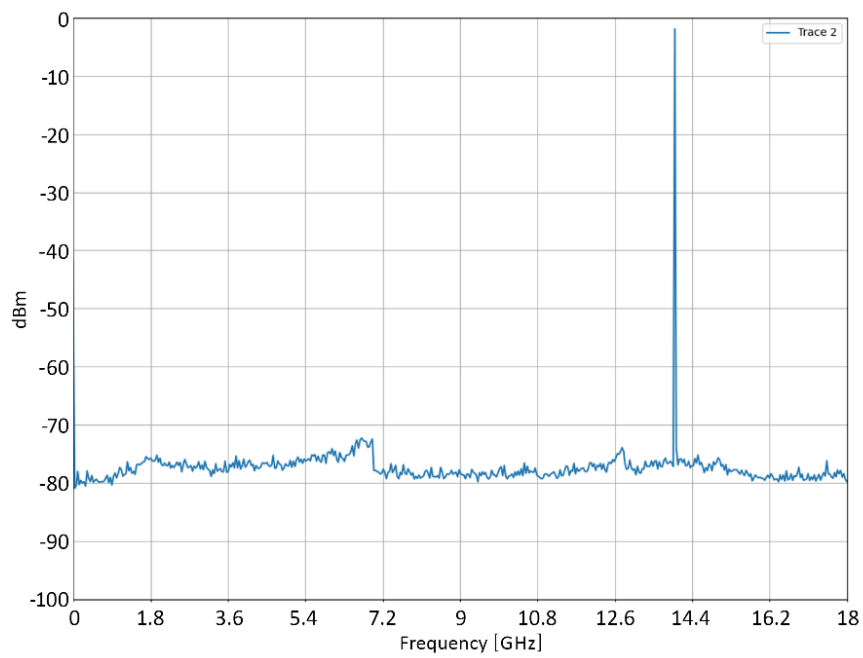
Figure 5. Wideband spectrum for 14 GHz
