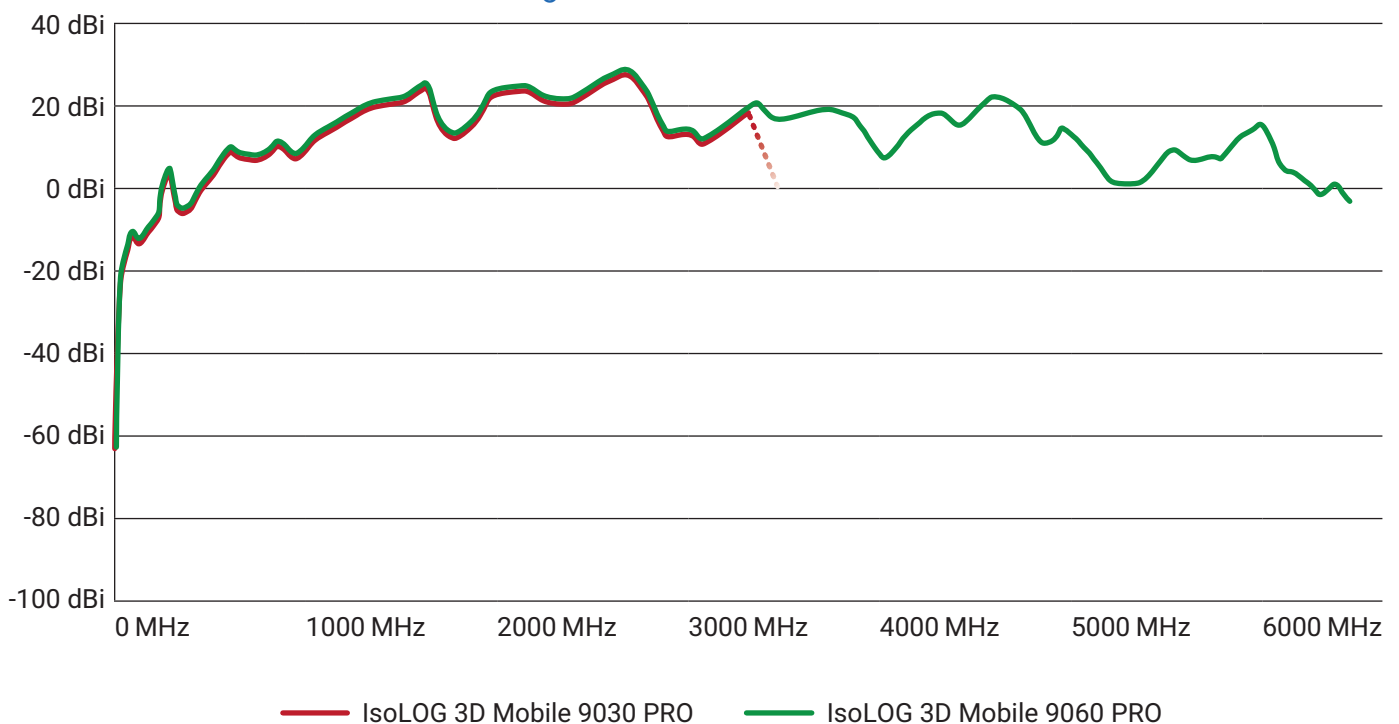
Gain Diagram IsoLOG® Mobile Antennas
