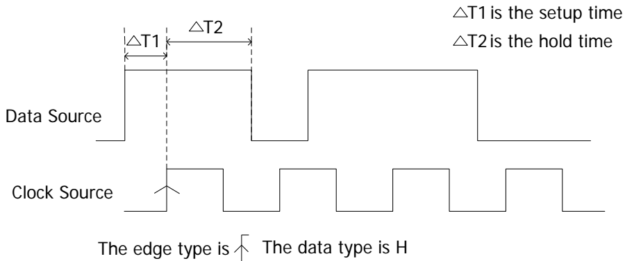
Figure 5-11 Setup/Hold Trigger
