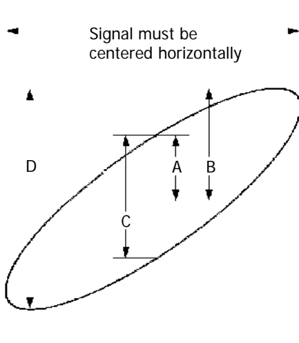
Figure 4-1 Measurement Schematic Diagram of Phase Deviation
