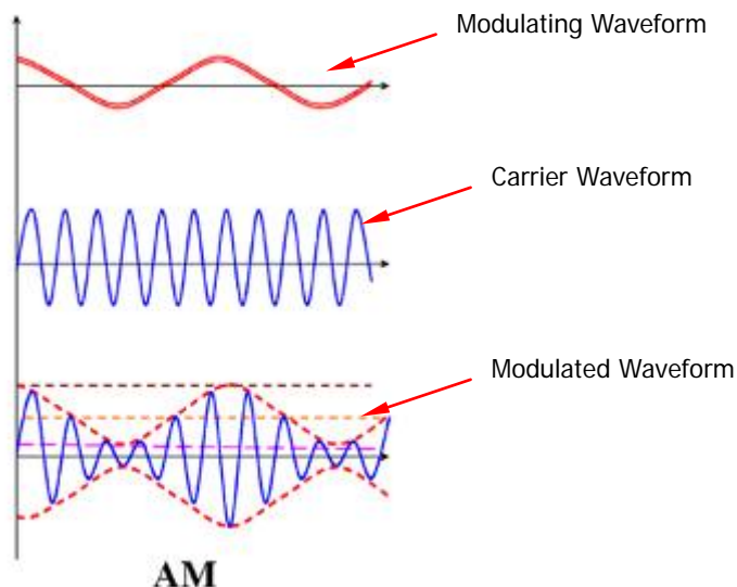
Figure 13-9 Amplitude Modulation
