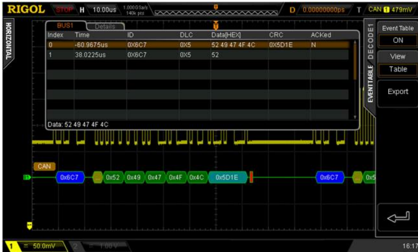
Figure 7-13 CAN Event Table (Table)
