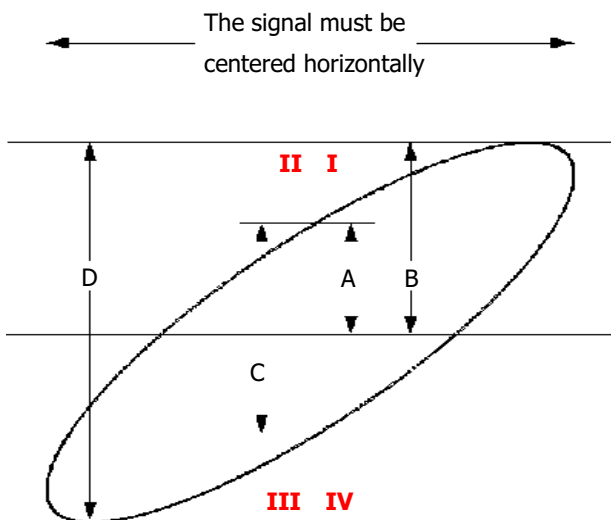
Figure 3-2 Measurement Schematic Diagram of Phase Deviation
