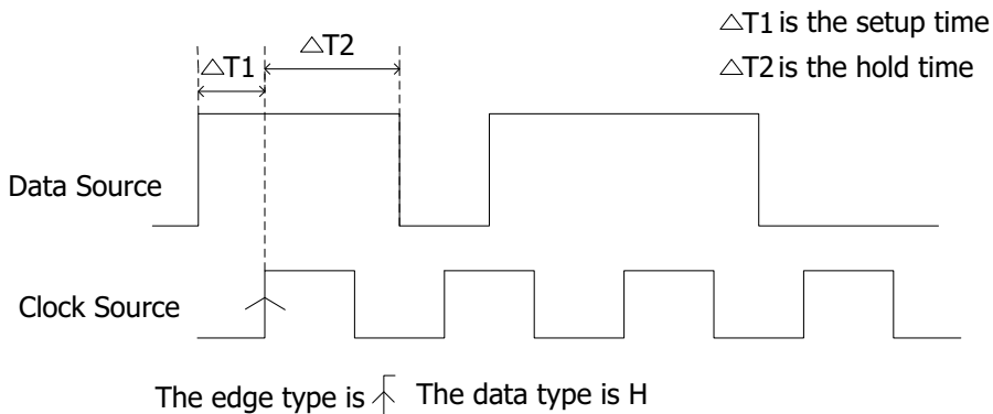
Figure 5-12 Setup/Hold Trigger
