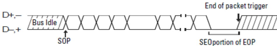
Figure 5-16 USB data transmission protocol diagram
