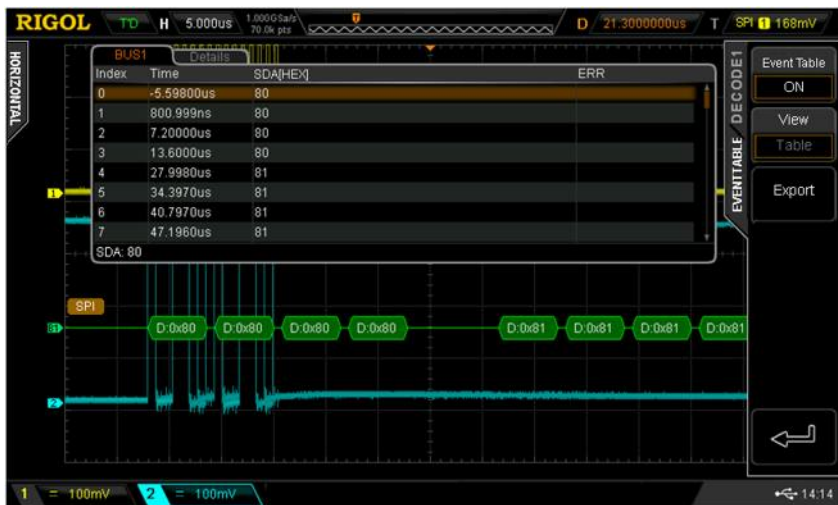
Figure 7-11 SPI Event Table
