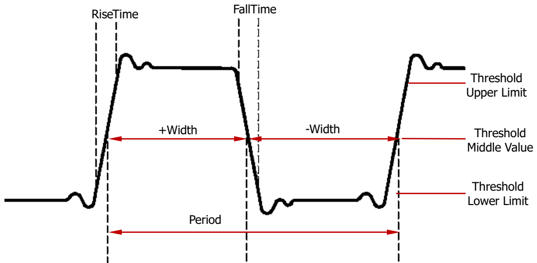
Figure 6-3 Time Parameters
