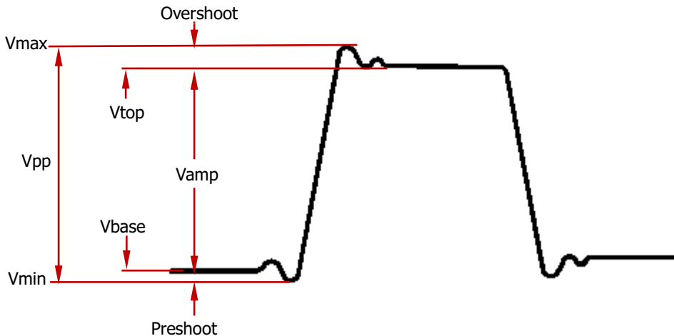
Figure 6-5 Voltage Parameters
