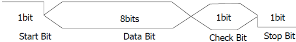
Figure 5-13 RS232 protocol diagram
