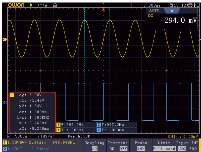
Figure 4-17 Time&Voltage Cursor Measurement
