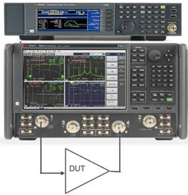
Classic NPR measurement with PNA-X and UTX
