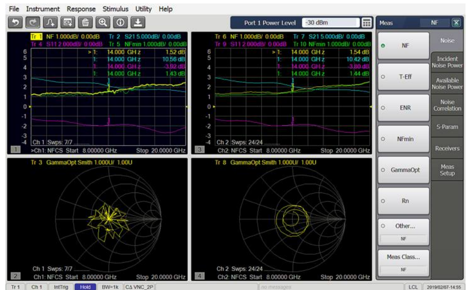
Unmatched device noise parameter measurements with ECal as impedance tuner vs with Maury LXI tuner as impedance tuner.
