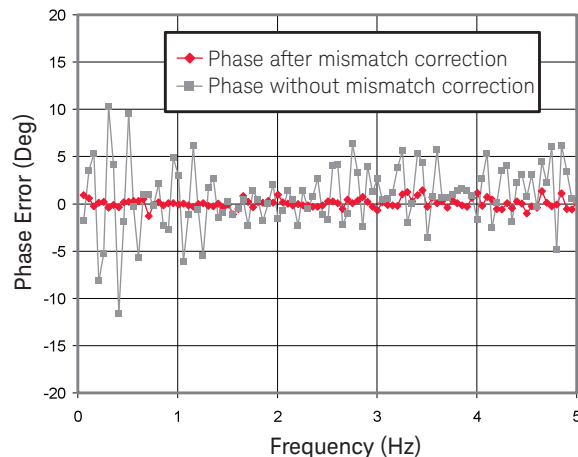
iTMSA compensates for mismatch errors by measuring the raw matches of the VNA and DUT, and precisely adjusting the amplitude and phase of the two signals at the reference plane to achieve ideal true-mode signals.
