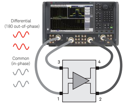
Using the PNA-X's two internal sources, iTMSA drives the differential amplifier under real world conditions, providing accurate mixed-mode S-parameters in all operating environments.
