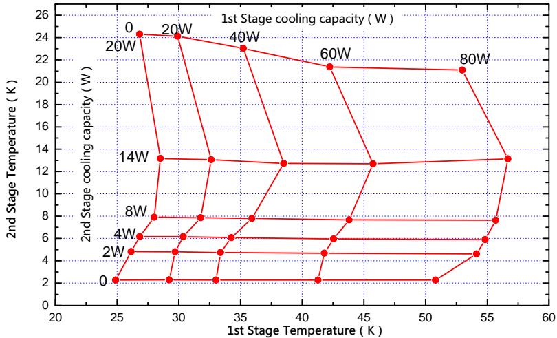
KDE410 Typical Load Map ( 50Hz )
